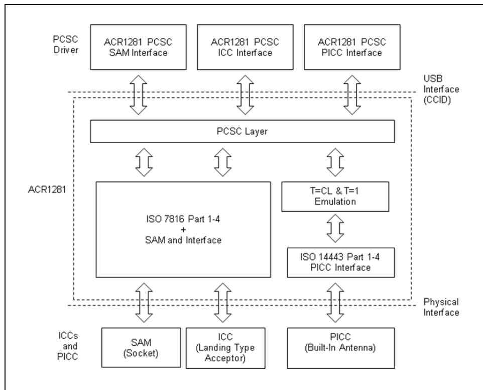
Figure 2: ACR1281U-C1 Architecture
