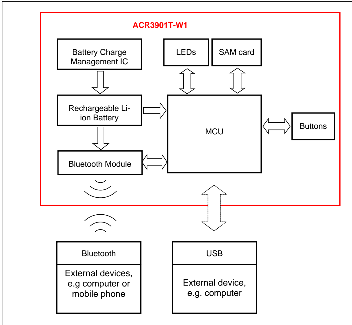
Figure 1: ACR3901T-W1 Architecture
