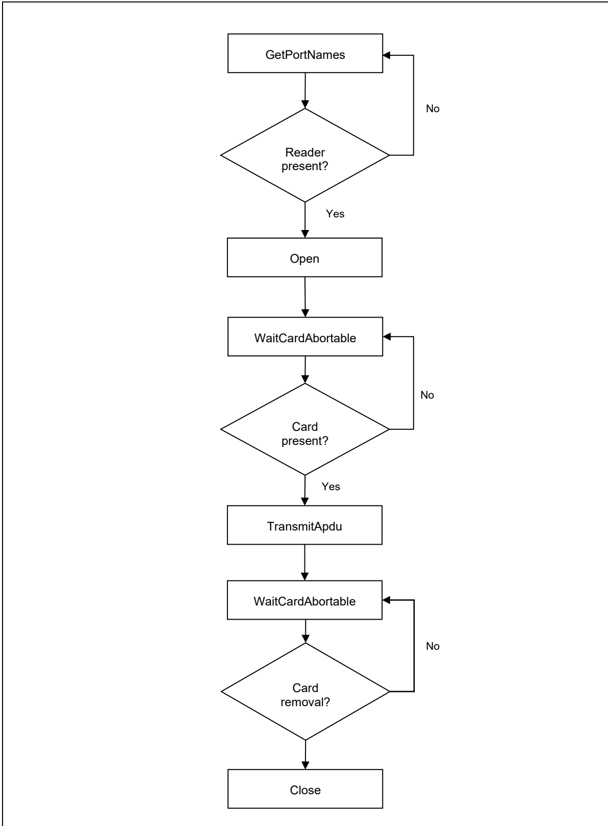
Figure 1: WalletMate II APDU Flow
